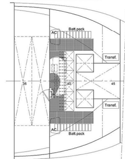
Arrangement Battery / Switchboard room
